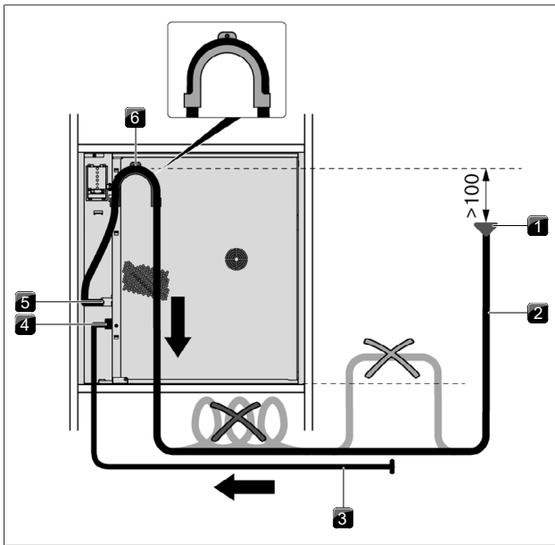
Fig. 9.12 Water drainage via hook
