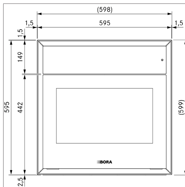
Fig. 3.1 X BO front view
