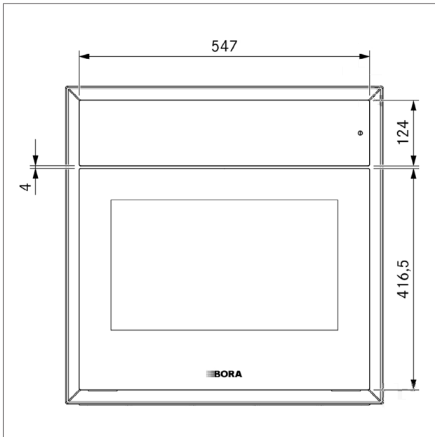
Fig. 3.4 XBO glass front view
