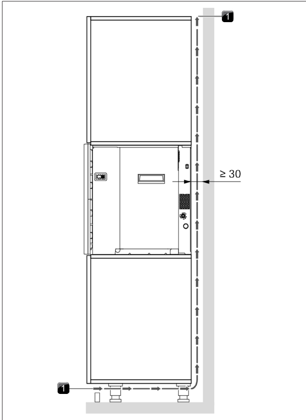
Fig. 9.16 Ventilation
