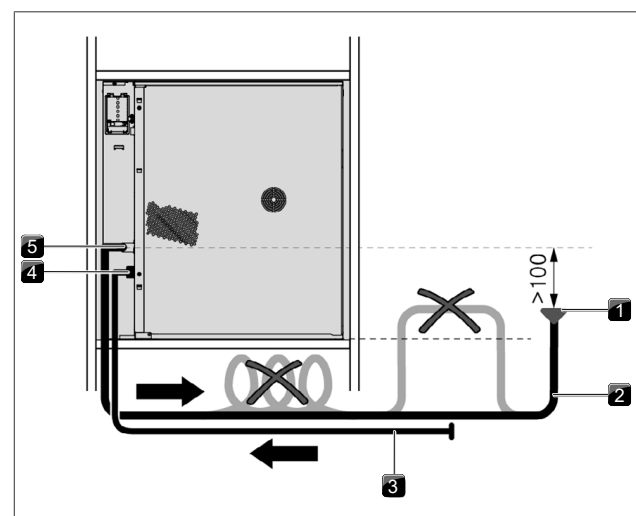
Fig. 9.11 Water drainage
