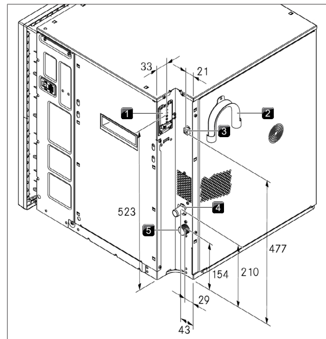
Fig. 9.10 Appliance connections
