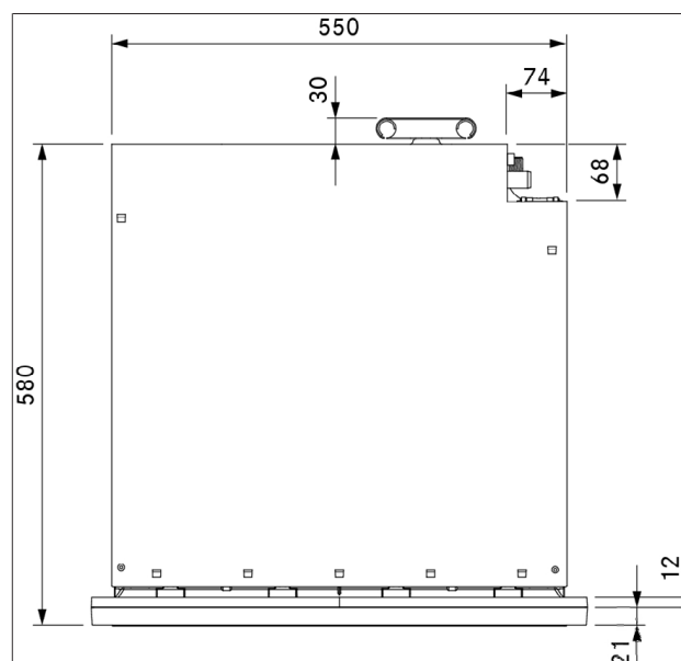
Fig. 3.2 X BO top view
