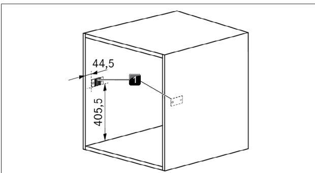
Fig. 9.9 Installation recess with unit mounting plates
