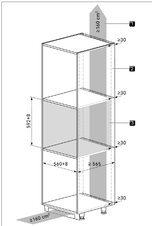
Fig. 9.1 Fitted unit
