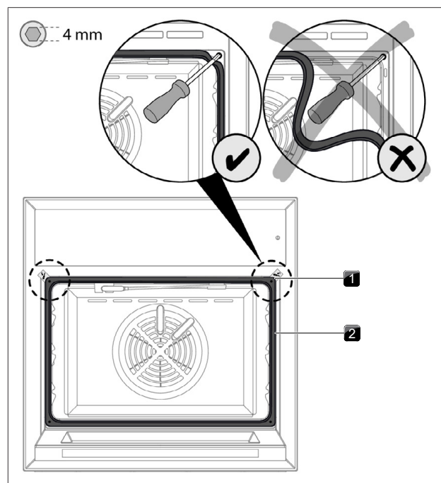
Fig. 9.15 Securing the appliance
