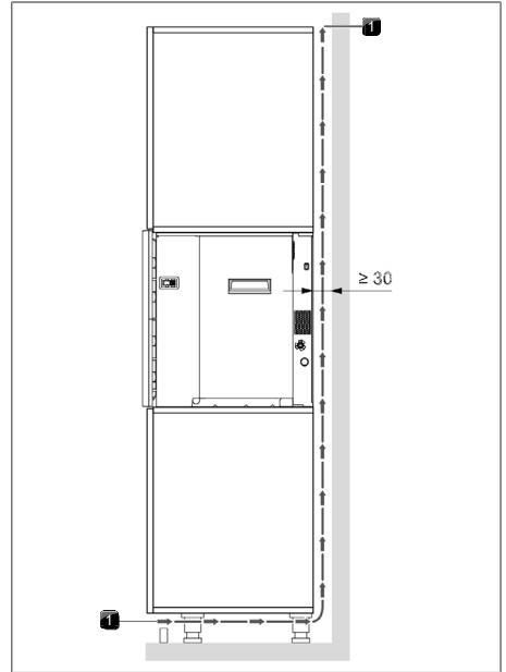
Fig. 9.17 Ventilation
